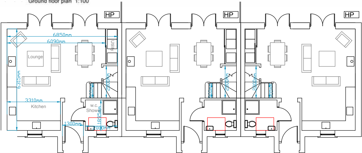
Ground floor plan 1:100
