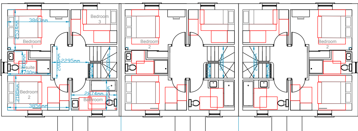
Proposed upper floor plan 1:100
