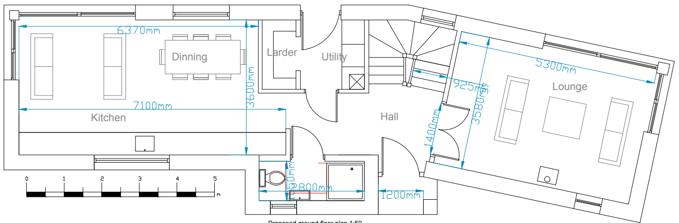
Proposed ground floor plan 1:50
